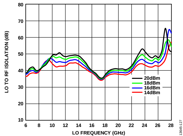
Figure 119. LO to RF Isolation vs. LO Frequency at Various LO Drives, IF = 100 MHz, T_A = 25^\circ\text{C}
