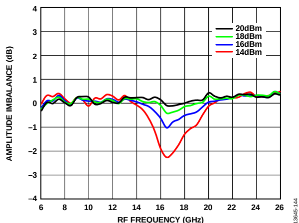
Figure 136. Amplitude Imbalance vs. RF Frequency at Various LO Drives, IF = 100 MHz, T_A = 25^\circ\text{C}
