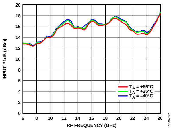
Figure 33. Input P1dB vs. RF Frequency at Various Temperatures, LO Drive = 18 dBm
