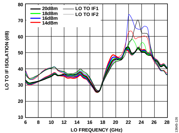
Figure 118. LO to IF Isolation vs. LO Frequency at Various LO Drives, IF = 100 MHz, T_A = 25^\circ\text{C}
