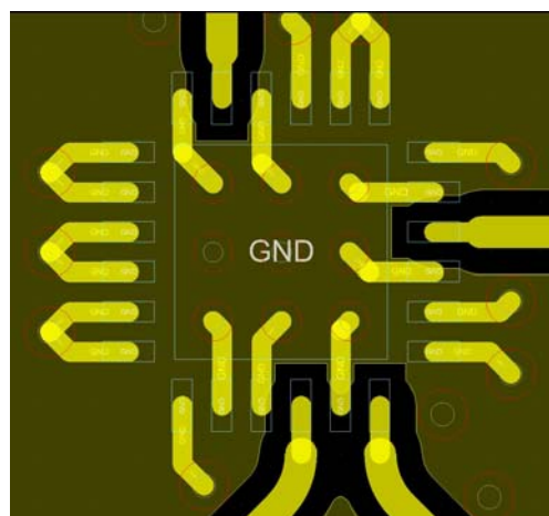
Figure 155. Evaluation Board Layout for the HMC8191 Package
