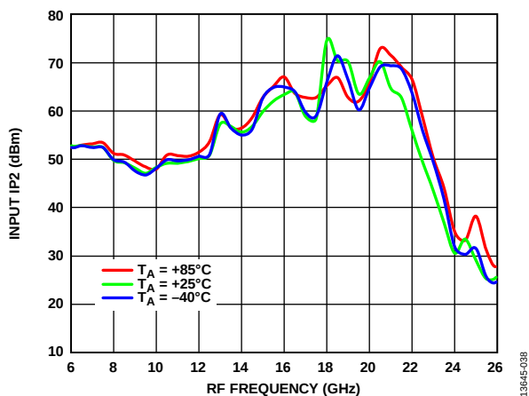
Figure 34. Input IP2 vs. RF Frequency at Various Temperatures, LO Drive = 18 dBm
