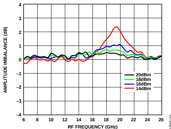
Figure 146. Amplitude Imbalance vs. RF Frequency at Various LO Drives, IF = 2500 MHz, T_A = 25^\circ\text{C}
