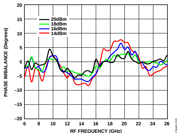
Figure 145. Phase Imbalance vs. RF Frequency at Various LO Drives, IF = 100 MHz, T_A = 25^\circ\text{C}
