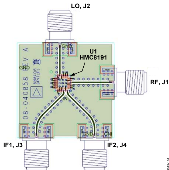
Figure 156. EV1HMC8191LC4 Evaluation Board PCB, Top Layer
