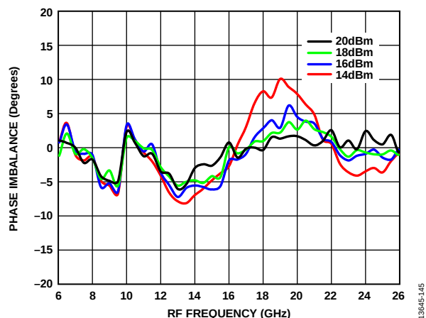
Figure 137. Phase Imbalance vs. RF Frequency at Various LO Drives, IF = 100 MHz, T_A = 25^\circ\text{C}
