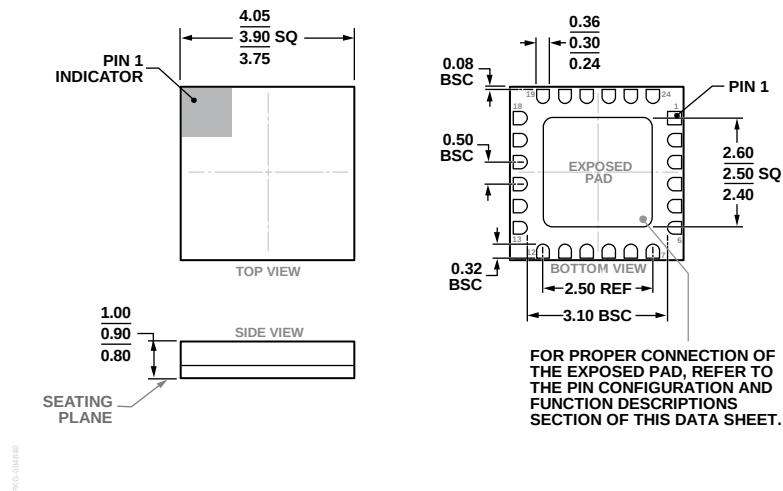
Figure 157. 24-Terminal Ceramic Leadless Chip Carrier [LCC] (E-24-1)
