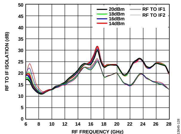
Figure 120. RF to IF Isolation vs. RF Frequency at Various LO Drives, IF = 100 MHz, T_A = 25^\circ\text{C}
