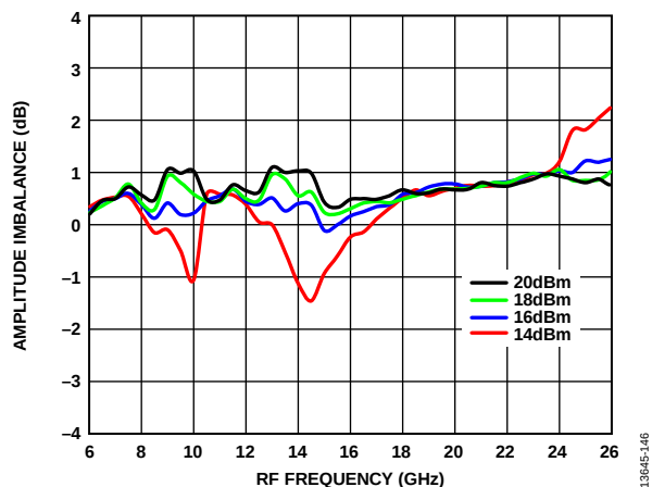
Figure 138. Amplitude Imbalance vs. RF Frequency at Various LO Drives, IF = 2500 MHz, T_A = 25^\circ\text{C}
